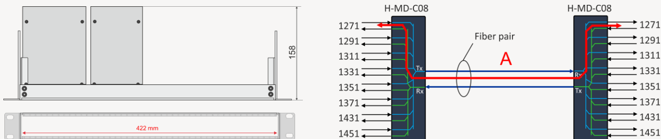
Mounting bracket dimensions with two example filters.
