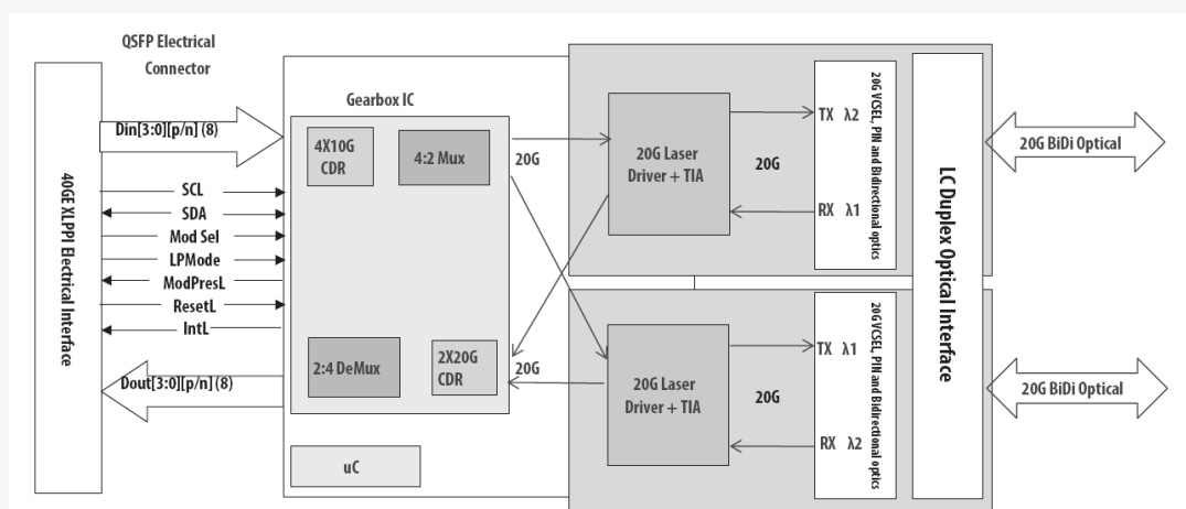
Transceiver Block Diagram
